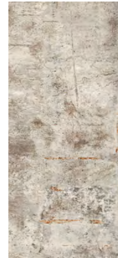
PLASTER
